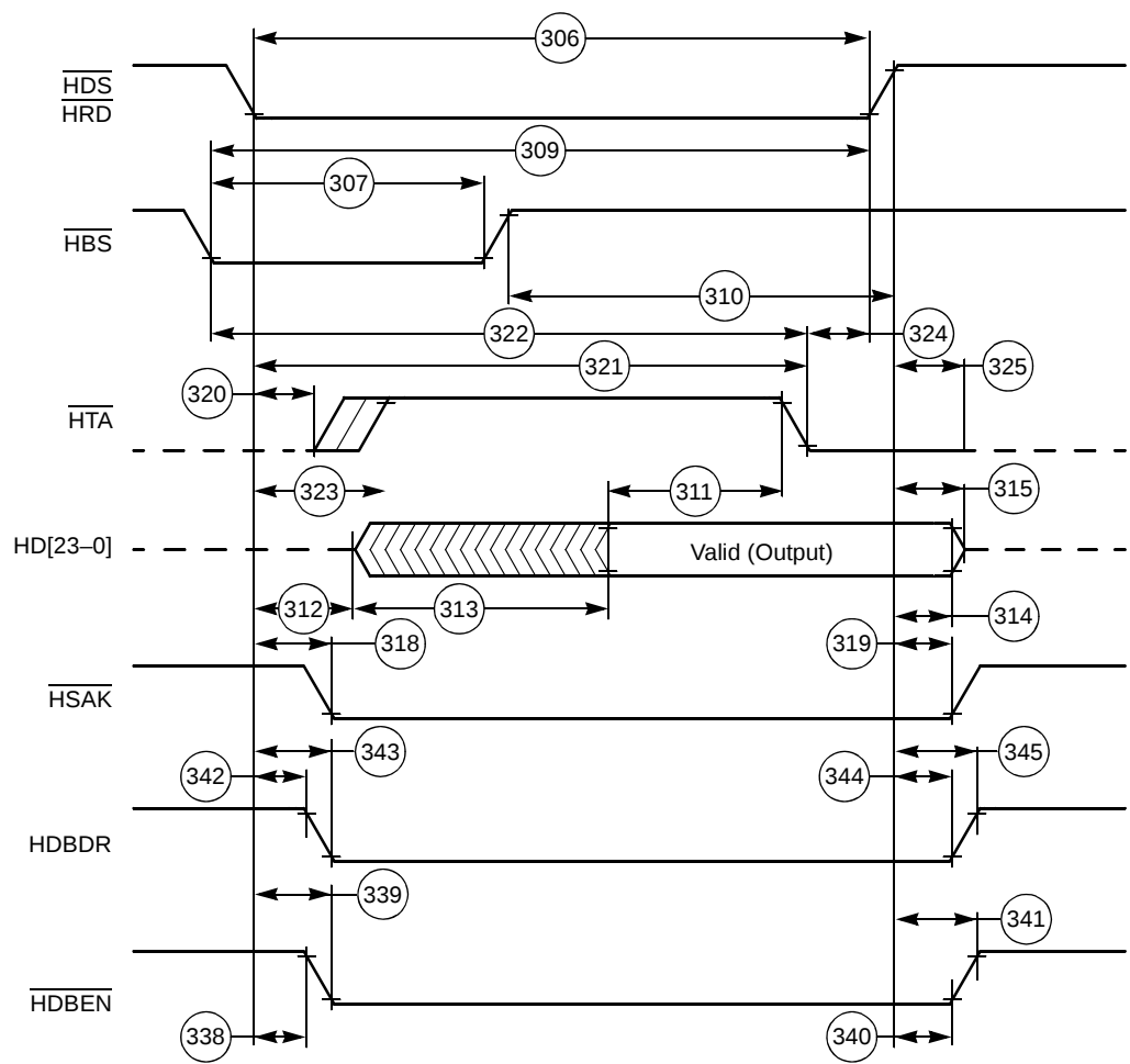
Figure 2-32. Read Timing
